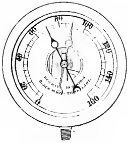
Fig. 1718. Duplex Air Gauge.
